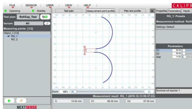
CALIPRI PORTABLE OPERATOR
