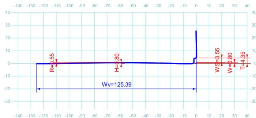
Measurement method “BrakeDisc” straight reference edge
