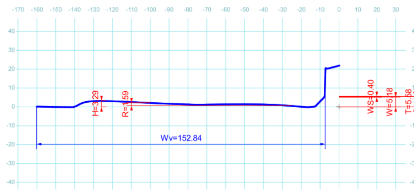
Measurement method “BrakeDisc” bevel reference edge
