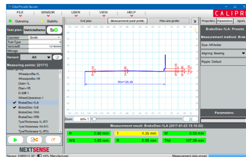
Measurement results on tablet-PC
