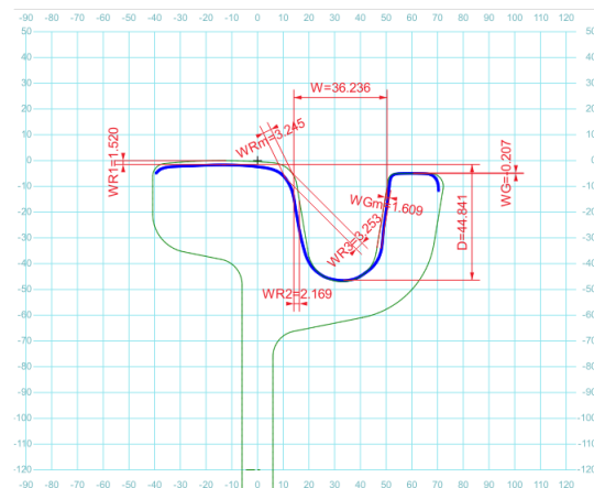
Messmethode "GroovedRailProfile"
