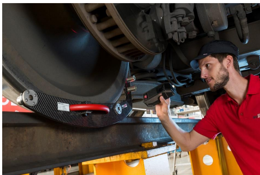
WHEEL DIAMETER MEASUREMENT WITH SENSOR AND G-GAUGE
